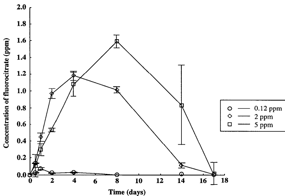
Figure 3. Formation and persistence of fluorocitrate with time in stream water aquaria. Error bars are \pm 1 standard error.
